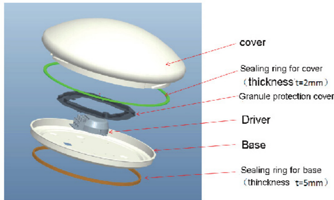
IP44 explosive view
